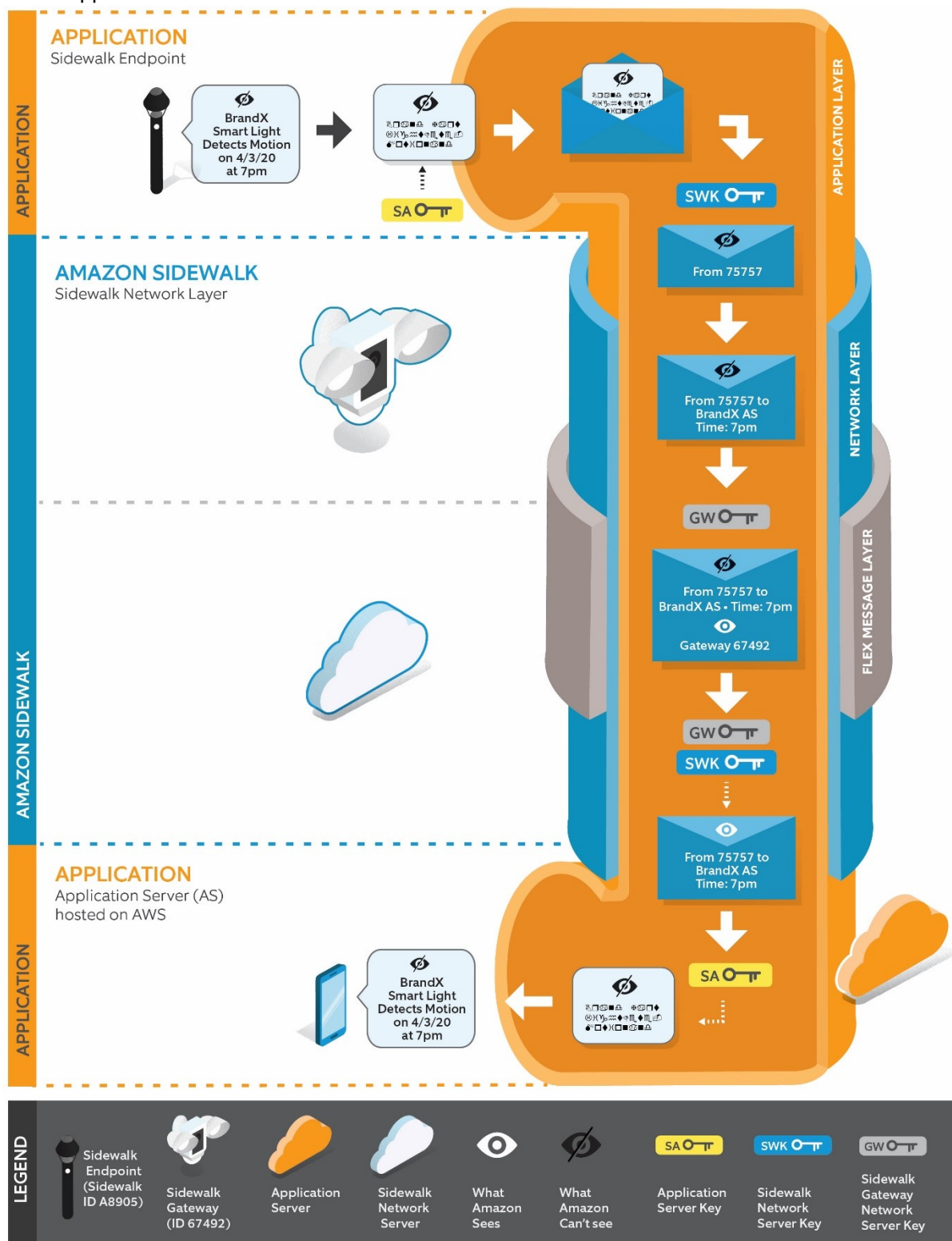
Figure 5: Endpoint Packet to Application Server
